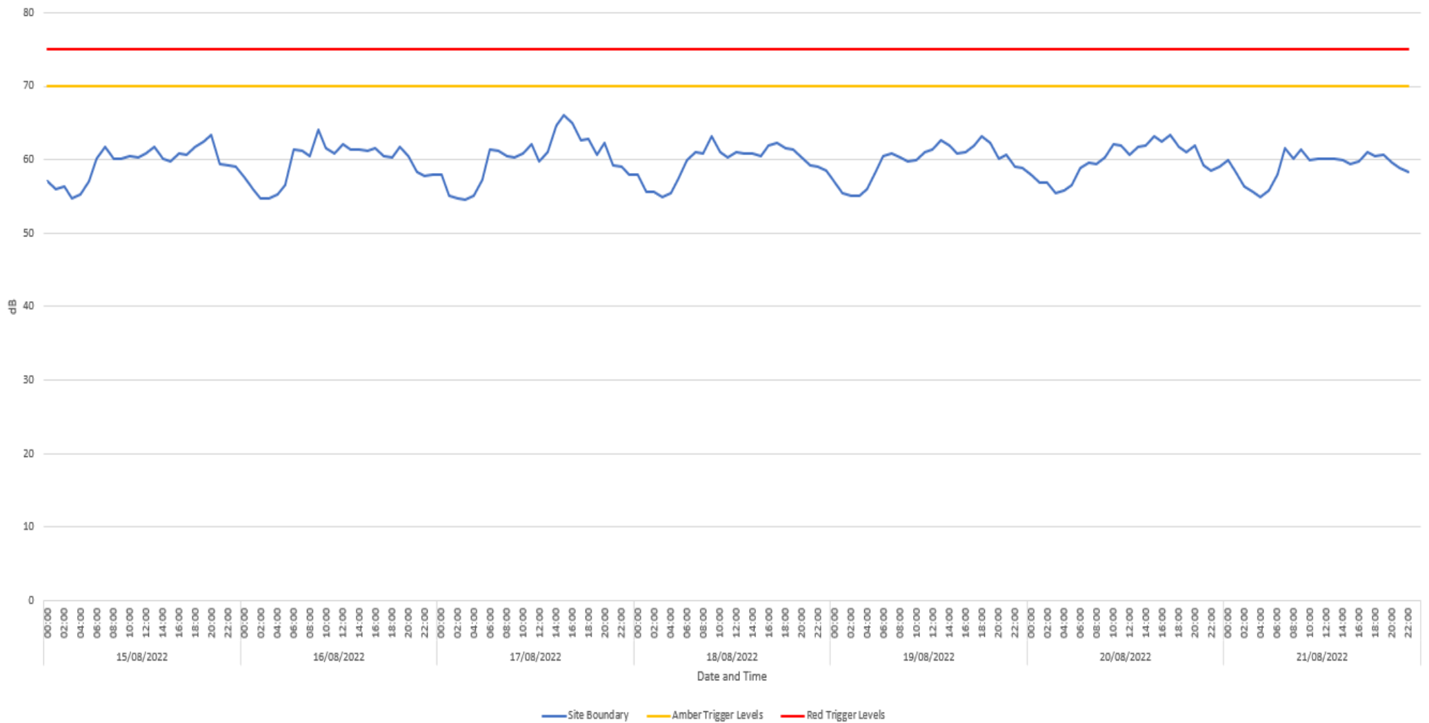
Figure 1. Noise Monitoring (15.08.22-21.08.22)
