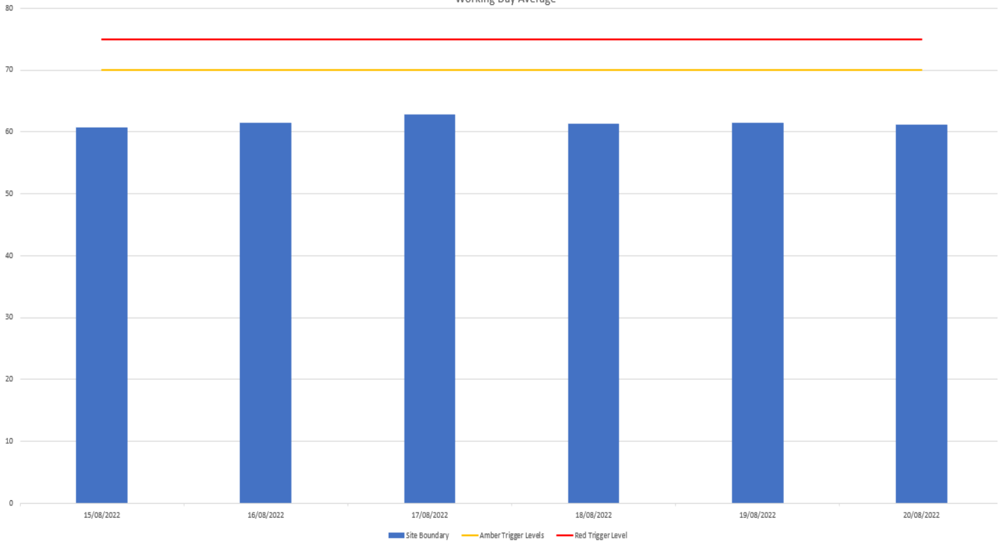
Figure 2. Noise Monitoring Working Hour Averages (15.08.22-21.08.22) – No exceedances.
