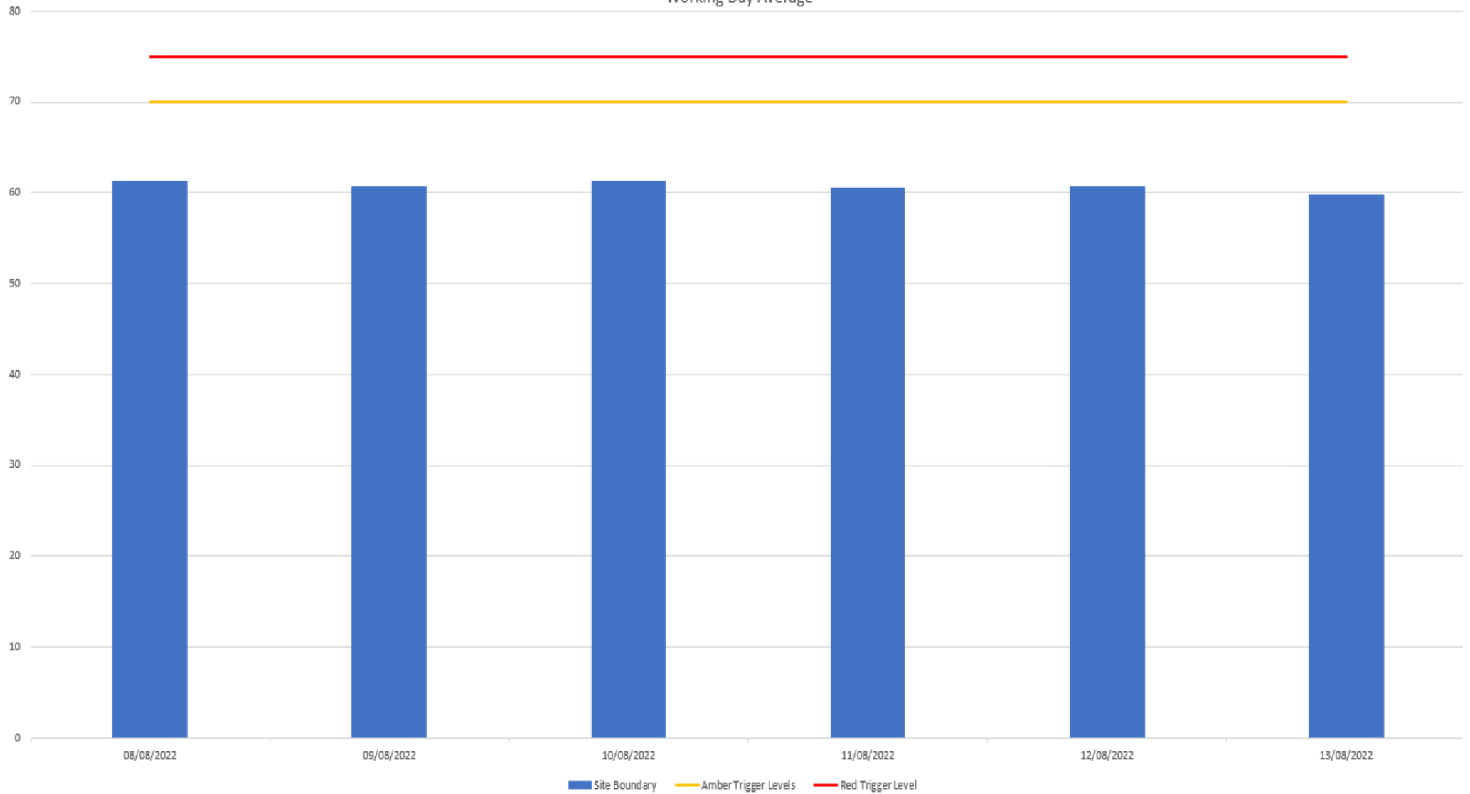
Figure 2. Noise Monitoring Working Hour Averages (08.08.22-14.08.22) – No exceedances.
