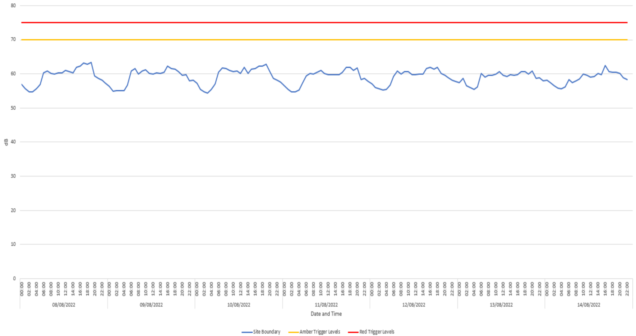
Figure 1. Noise Monitoring (08.08.22-14.08.22)
