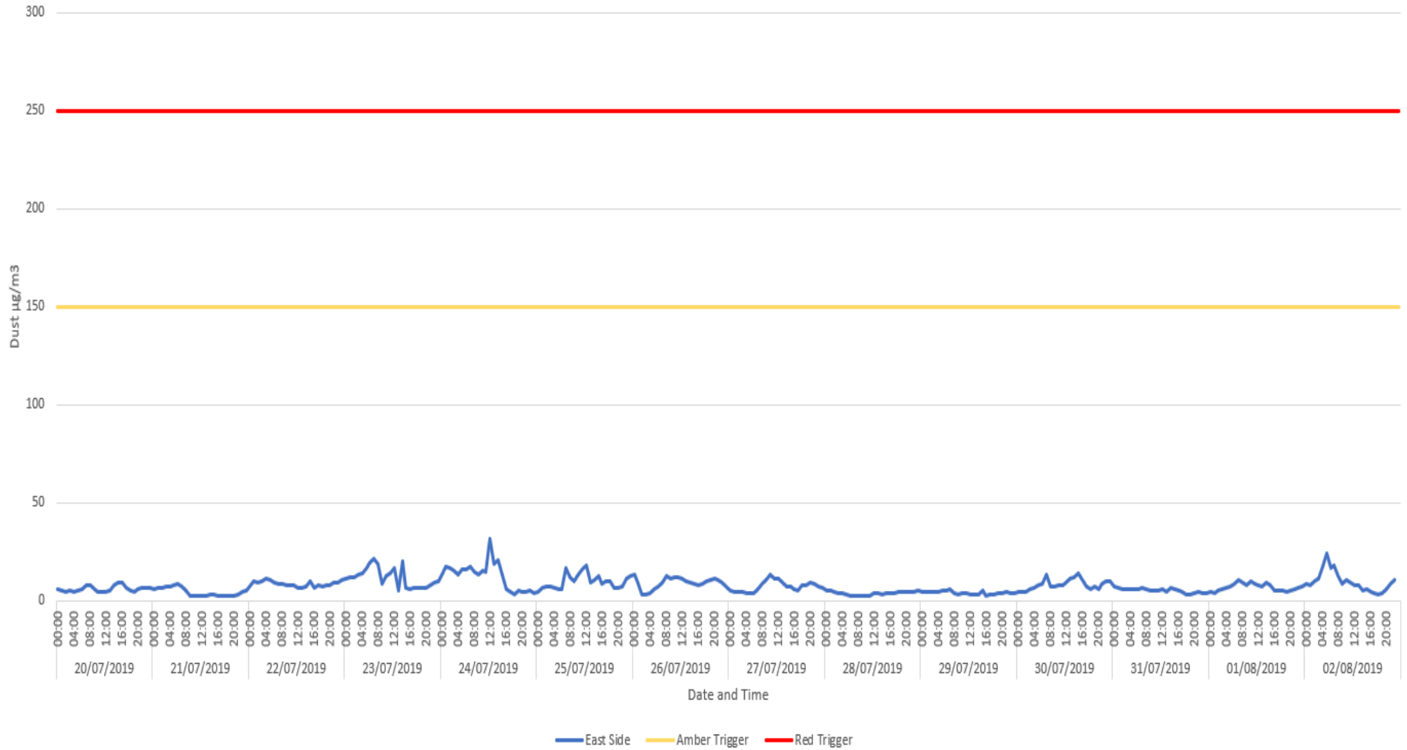
Figure 6. Air Quality Data East Side Boundary (Near Emergency Gate) – No Exceedances
