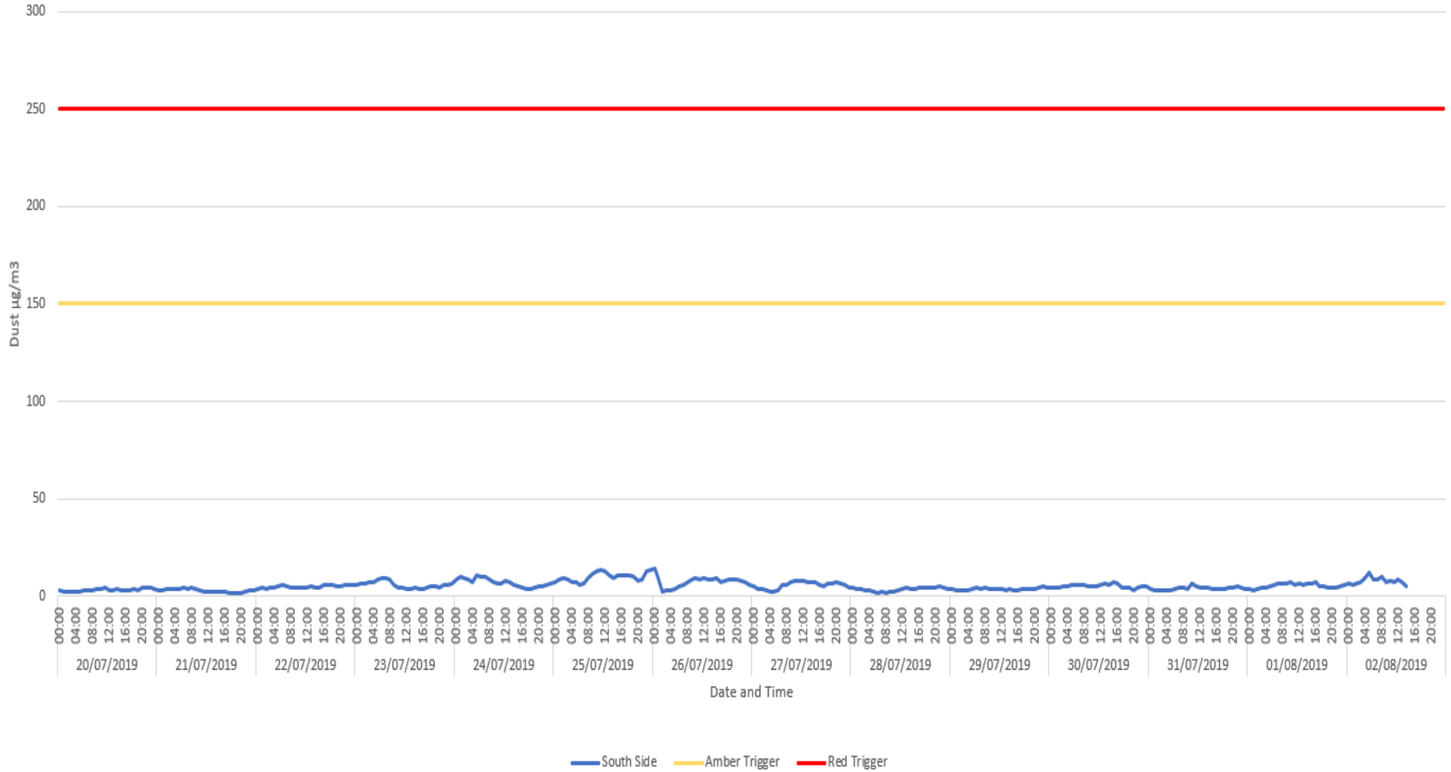
Figure 8. Air Quality Data South Side Boundary (Near Existing Sculpture) – No Exceedances
