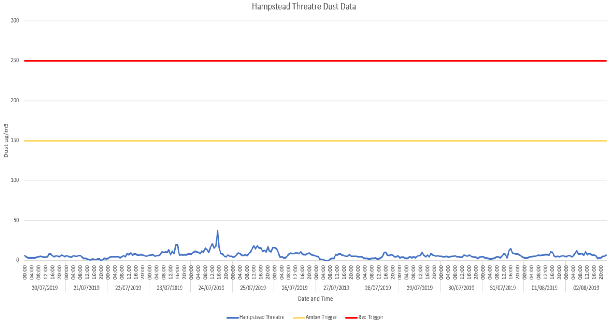
Figure 4. Air Quality Data Hampstead Theatre – No Exceedances
